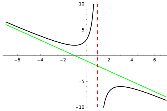
Figur 1: Kurvan f(x) = \frac{3 + x^2}{1 - x} .
